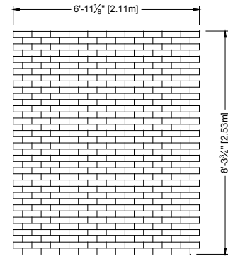
10-1-117 Offset Brick
