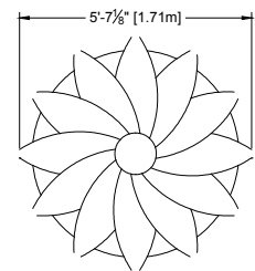
17-113 Pinwheel Insert
